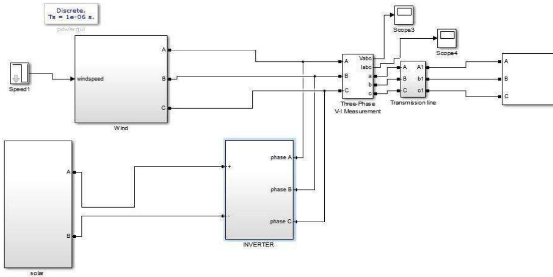
Fig 1.9 MODEL OF COMPLETE HYBRID SYSTEM CONNECTED TO GRID
