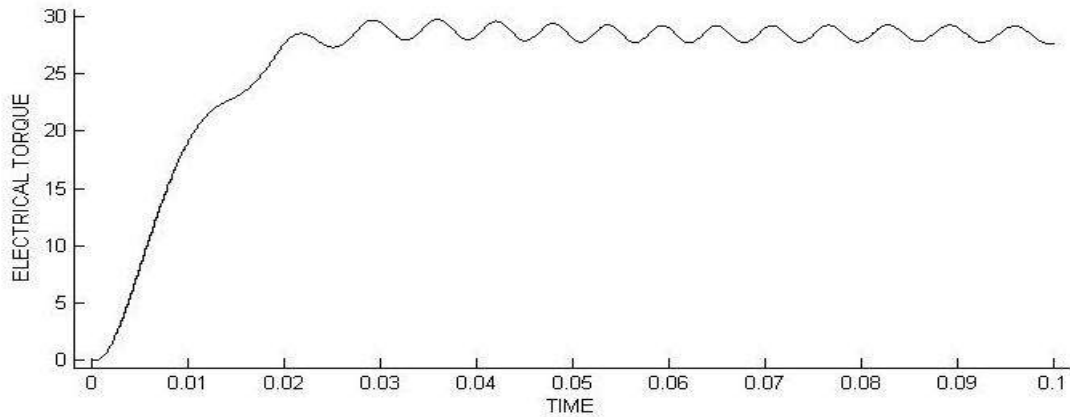
Fig 1.10 electrical torque developed by wind generator
