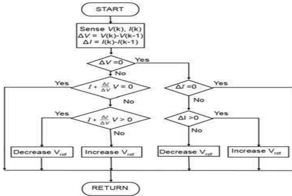
Fig. 1.7: Incremental Conductance algorithm flow chart.
