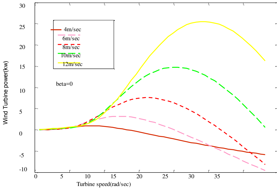
Fig.1.5 Characteristics of power vs speed with different wind speed
