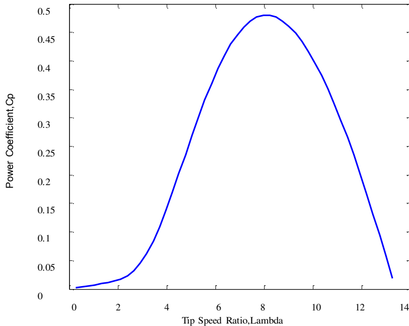
Fig.1.3 Characteristics of C_p vs \lambda curve
