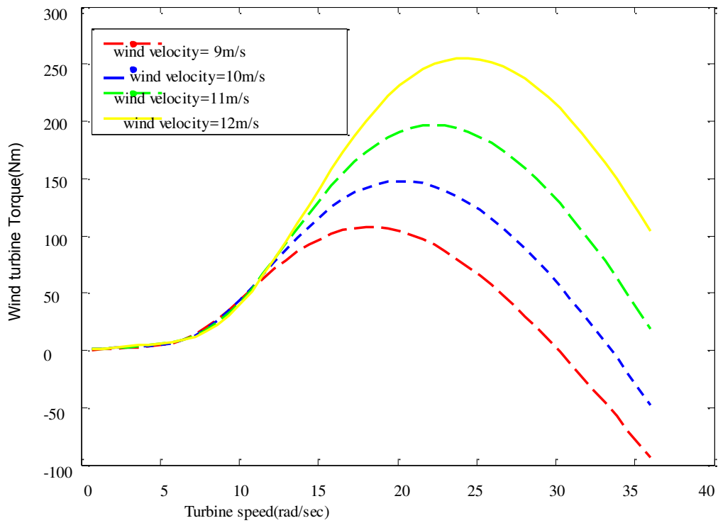
Fig.1.4 Characteristics of torque vs speed with different wind speed
