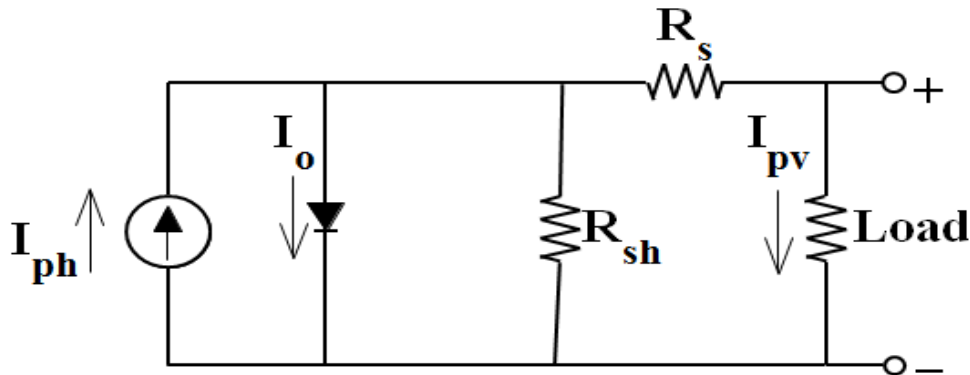
Fig.1.2 Circuit diagram of a single PV cell
