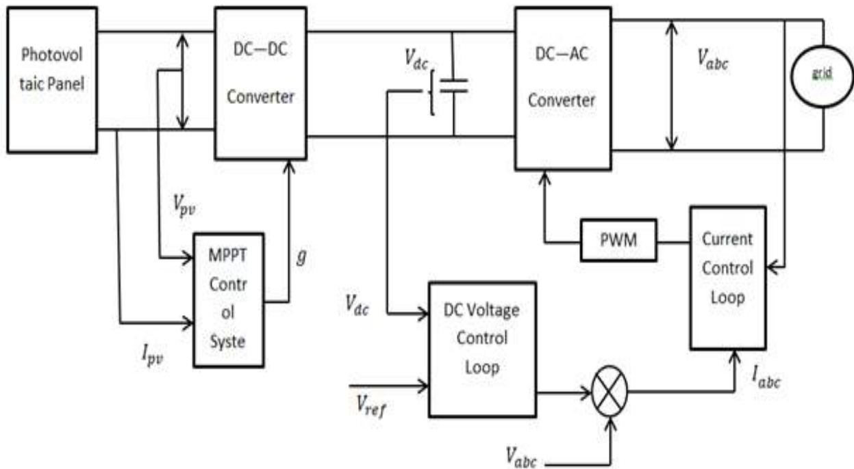
Fig.1.8 Control Strategy to connect the PV system with Grid
