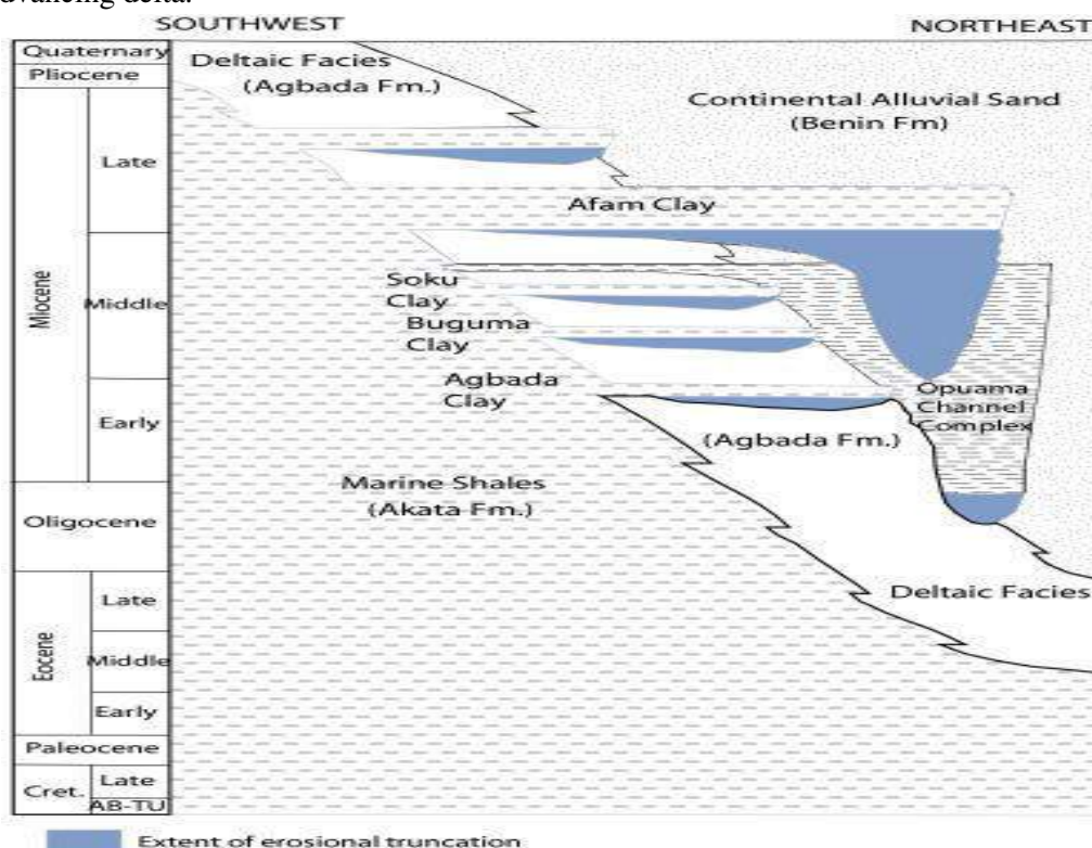
Figure 1 : Stratigraphic column showing the three formations of the Niger Delta. (Adapted From: Tuttle et al, 1999).
