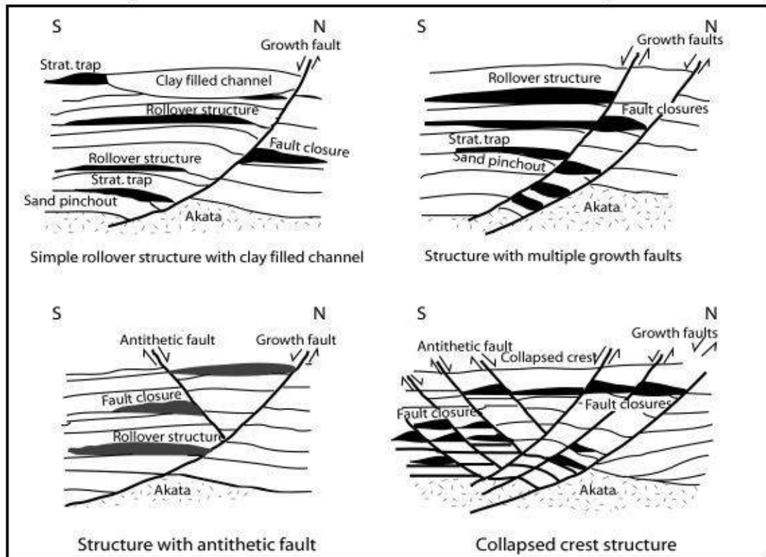
Figure 2: Major structures and associated traps in the Niger Delta.
