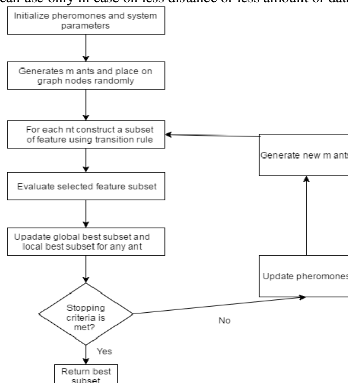
Figure 1. Flow chart of ant colony optimization
