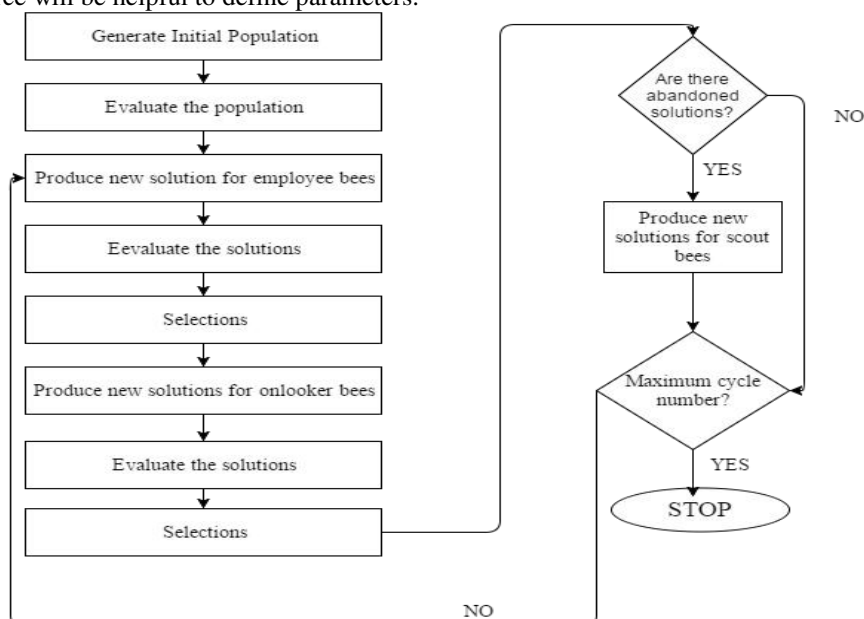
Figur 2. Flowchart of artificial bee colony optimization
