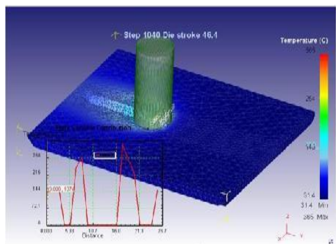
Fig 6.4: Temperature distribution during welding
