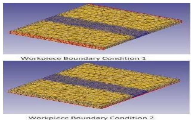
Fig 6.2 Work piece boundary conditions
