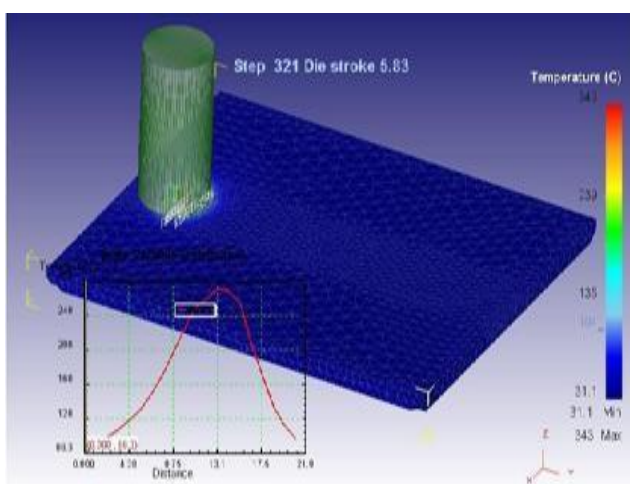
Fig 6.3 Temperature distribution during plunging step 1040
