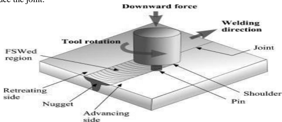
Fig.1.1 Schematic drawing of FSW process
