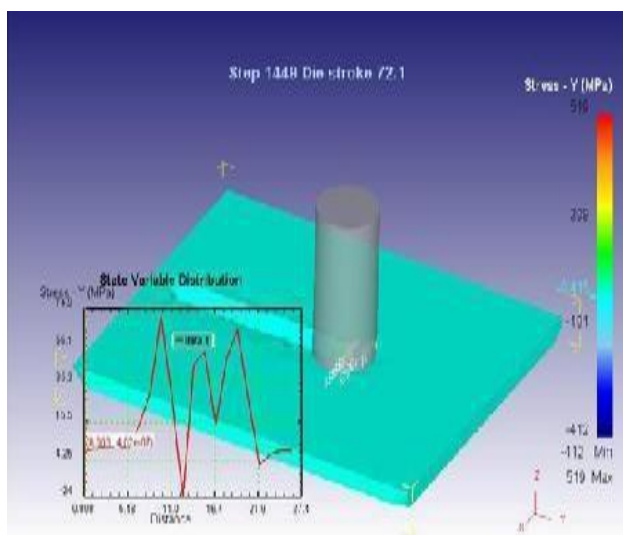
Fig 6.7 Longitudinal stress distribution during welding at 1340 rpm
