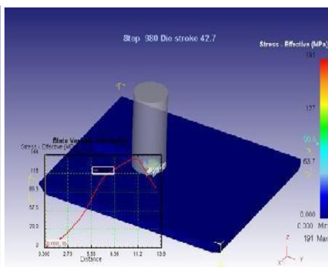
Fig 6.6 Effective stress distribution during welding phase 1340 rpm
