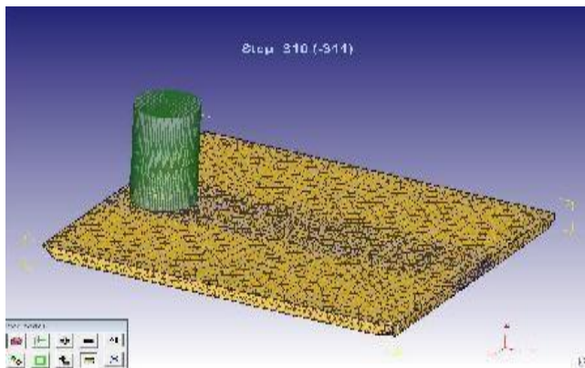
Fig 6.1 Meshed model in DEFORM-3D
