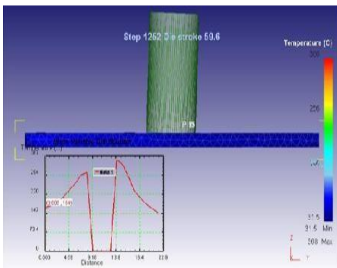
Fig 6.5: X- Direction temperature distribution
